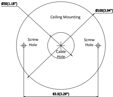
Figure 2-22 Drill Template
